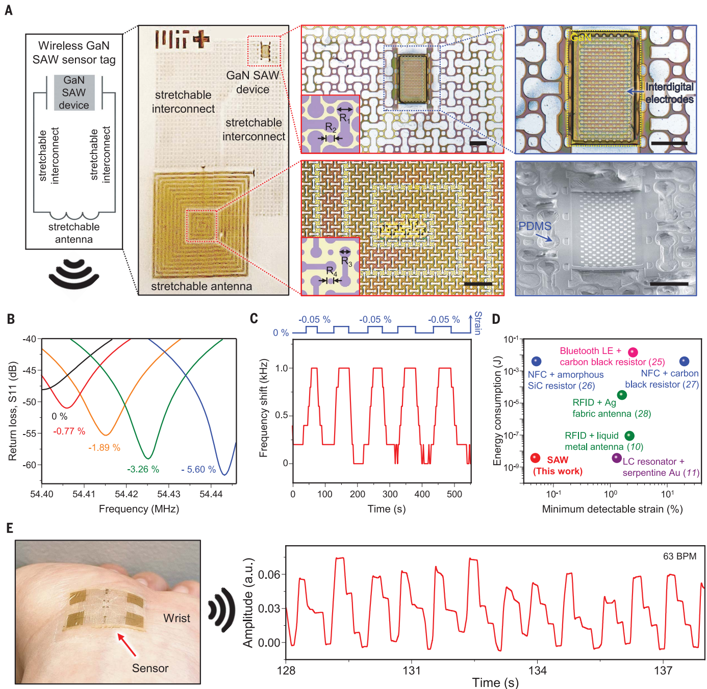
Fig. 3. Wireless GaN SAW strain sensors on e-skins free of communication chips or power source. (A) Schematic illustration and optical images of our wireless GaN SAW e-skin strain sensor. R1, R2, R3, and R4 in insets are 120, 50, 20, and 10 \mu\text{m} , respectively. Scale bars, 200 \mu\text{m} . (B) Resonant frequency shift as a function of strain for GaN SAW e-skin strain sensors.
